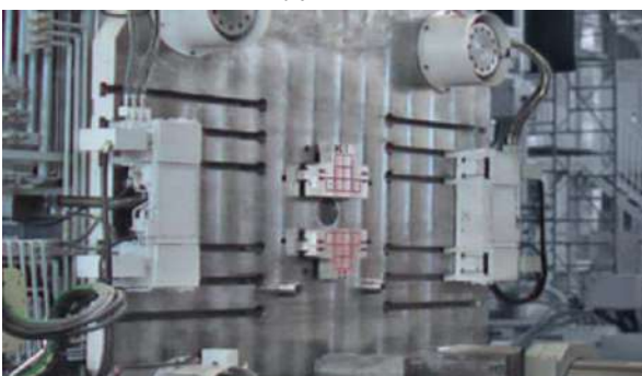
40,000kN (4,000ton) Mesin Die-casting plat-C klem magnet
