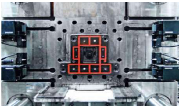
8,500kN (850ton) Mesin Die-casting plat-C klem magnet & Klem hidrolik TYB-Z
